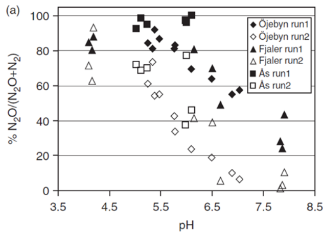
Fig. 2. Denitrification rates and gas product ratios [ N_2O:(N_2+N_2O) ] during anoxic incubation of soils from three liming experiments: Fjaler, Öjebyn and Ås. Product ratios (a) are expressed as molar % N_2O [ N_2O:(N_2+N_2O) ] and denitrification rates (b) are expressed as \mu g
